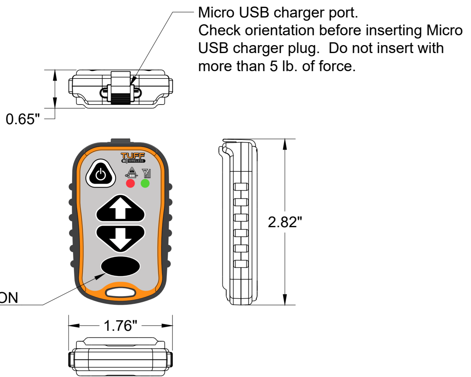
P/N: 3A577BA TRANSMITTER, MICRO, 3 BUTTON
